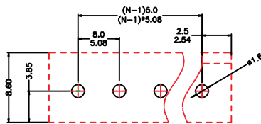
PCB LAYOUT(RECOMMENDED) (TOP VIEW TOL. :±0.05)
